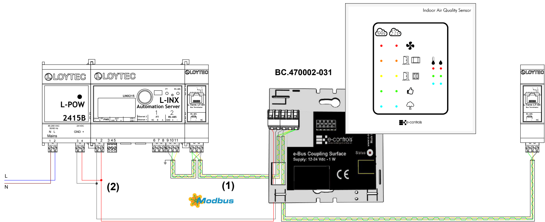
Instalación cableado bus RS-485. RS-485 bus wiring installation.
