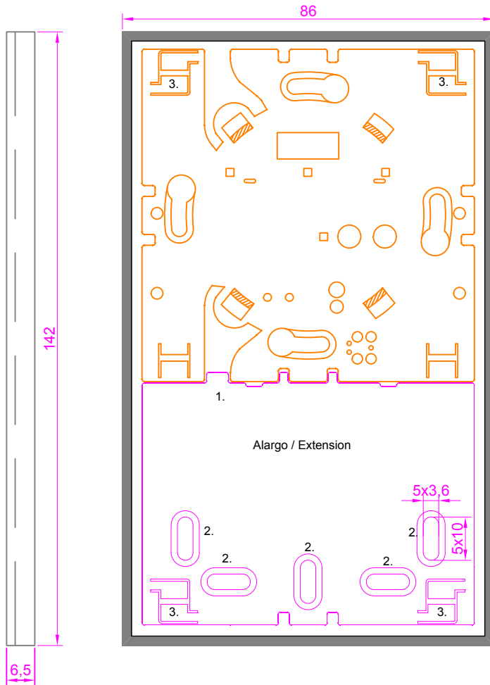
e-Bus coupling + extension + frame
